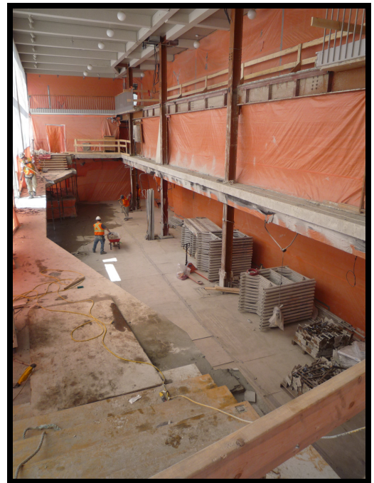
Selective structural demolition in dust enclosures & lead dust abatement
